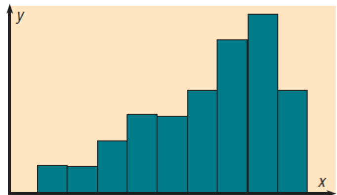
(f) Left-skewed
