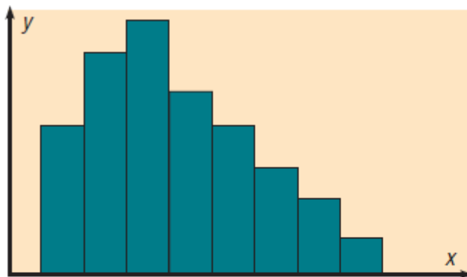
(e) Right-skewed
