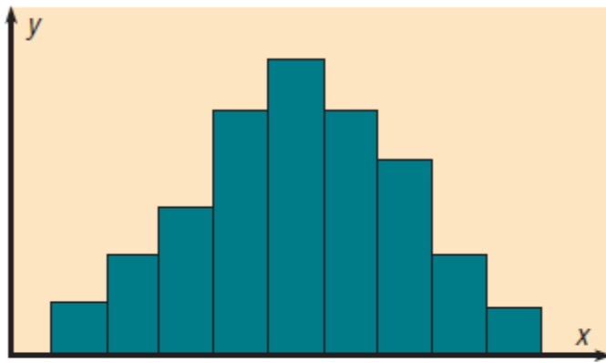
(a) Bell-shaped
