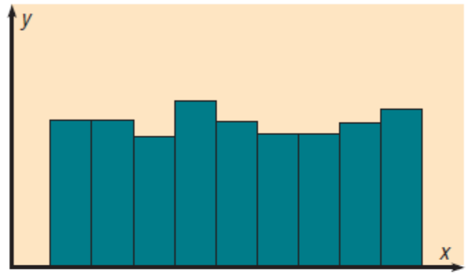
(b) Uniform
