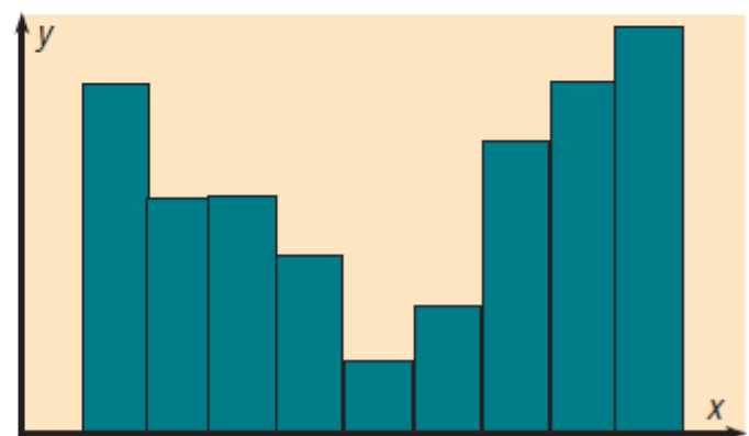
(h) U-shaped
