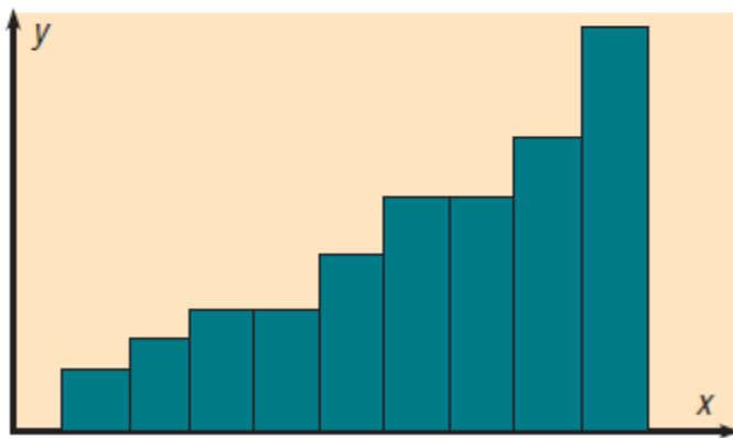
(c) J-shaped
