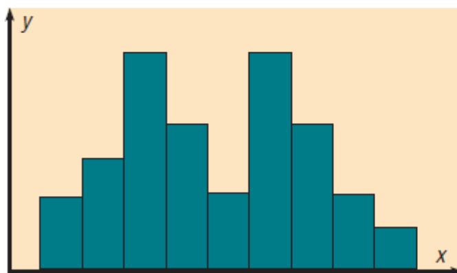
(g) Bimodal
